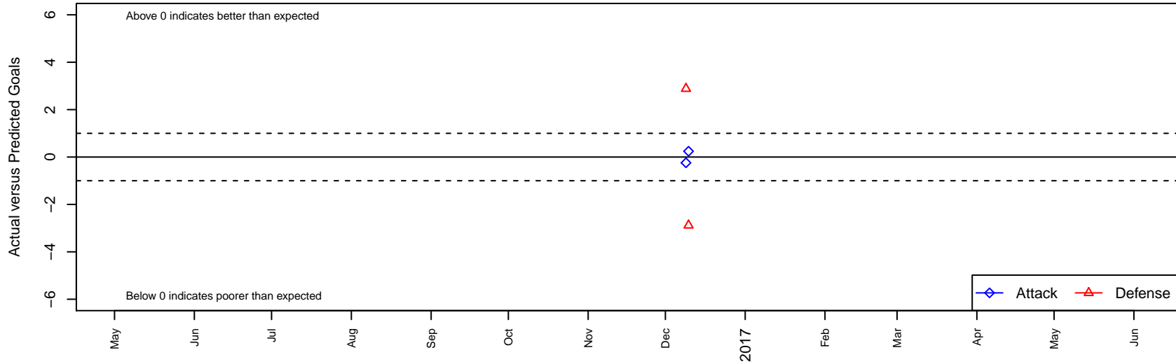
Showcase TBD B02 Dots are actual minus expected GF (blue circles) and GA (red triangles). Blue line is smoothed change in attack strength. Red is smoothed change in defense strength.
